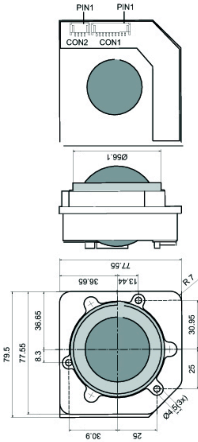
4 way connector (CON2) For PS/2 & USB only
